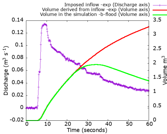
Figure 13. Hydrograph of the imposed inflow on the left boundary. Comparison of the volume of water in the simulation and the experimental one.
