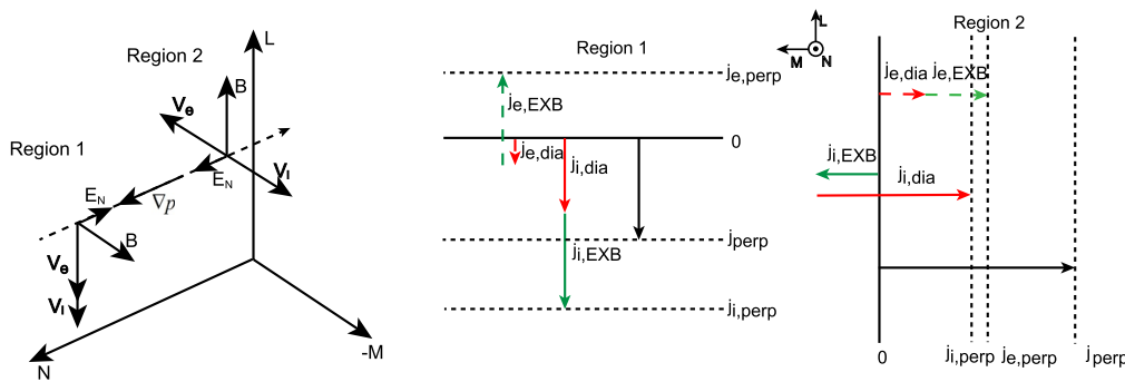
Figure 13. Top: Sources of a thin magnetopause current sheet calculated by MMS data. Bottom part: a schematic illustrator of all the vectors. (left) The vectors of magnetic field B , electric field E , plasma velocity V , cross-field drift E \times B , and gradient of pressure \nabla p in regions 1 and 2 and (middle and right) current distribution in region 1 and region 2. Note that region 1 and 2 here refer to the outer and inner magnetopause current sheet region, respectively. The Figure is adopted from Dong et al. (2018).
