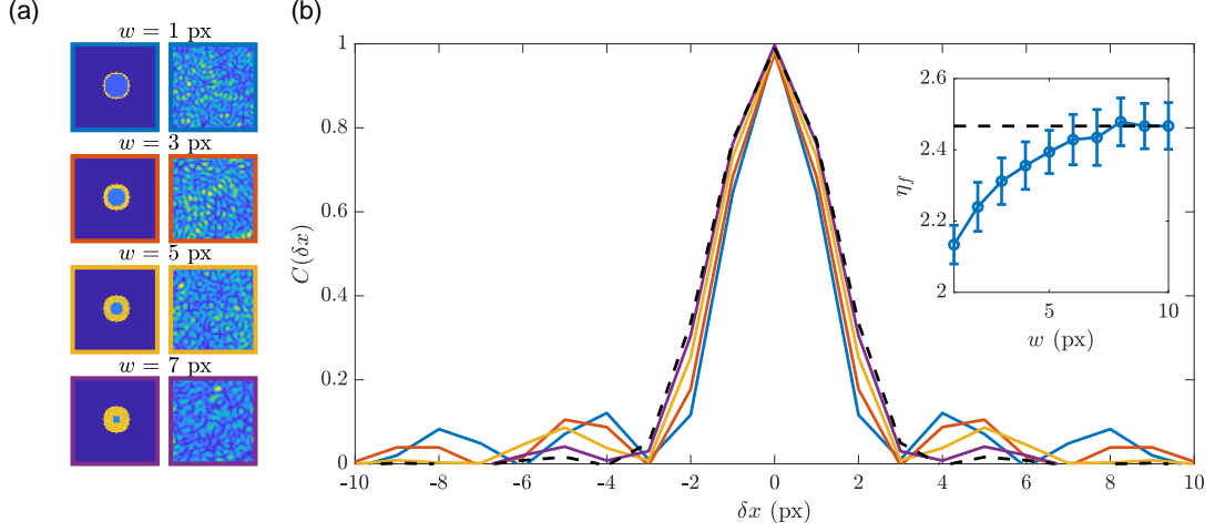
FIG. S5. Simulation of the filtering step impact on the noise. (a) Average Fourier transform of the fields behind the scattering medium (left) for different widths w of the filtering ring mask and examples of the associated speckles' field amplitudes (right). (b) Field autocorrelation (line colors correspond to the frame colors in (a)) and in inset the field enhancement of the first singular vector (No. 1) as a function of w for a complete set of masks. Error bars are given by the field enhancement standard deviation. The data are averaged over 50 realisations.
