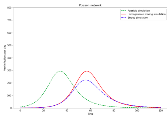
Figure 5: Daily incidence on a Poisson network of 10000 nodes with a mean degree of 10. The red, blue and green lines are results from compartment-based approaches: homogeneous, Stroud et al. and Aparicio et al. respectively.
