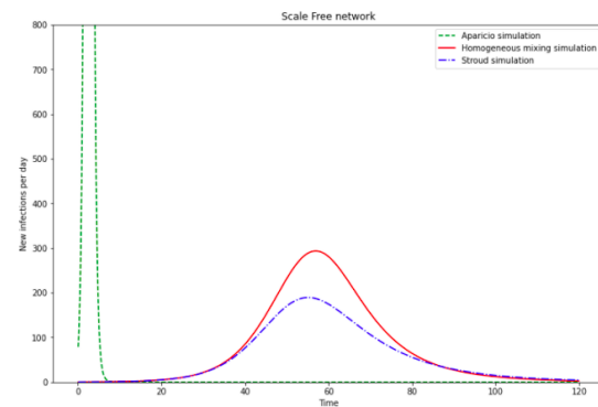
Figure 7: Daily incidence on a scale free network of 10000 nodes with a mean degree of 10. The red, blue and green lines are results from compartment-based approaches: homogeneous, Stroud et al. and Aparicio et al. respectively.
