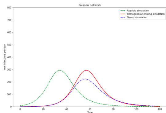
Figure 5: Daily incidence on a Poisson network of 10000 nodes with a mean degree of 10. The red, blue and green lines are results from compartment-based approaches: homogeneous, Stroud et al. and Aparicio et al. respectively.
