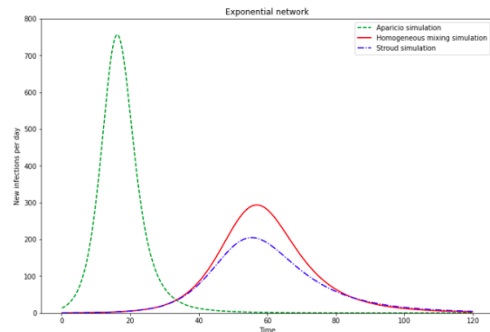
Figure 6: Daily incidence on an exponential network of 10000 nodes with a mean degree of 10. The red, blue and green lines are results from compartment-based approaches: homogeneous, Stroud et al. and Aparicio et al. respectively.
