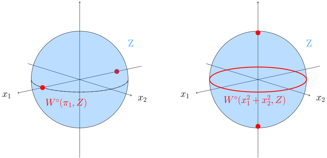
FIGURE 1: Real trace of the critical locus on a sphere Z for: the projection on the first coordinate \pi_1 (left); the polynomial map associated to x_1^2 + x_2^2 \in \mathbb{R}[x_1, x_2, x_3] (right).
