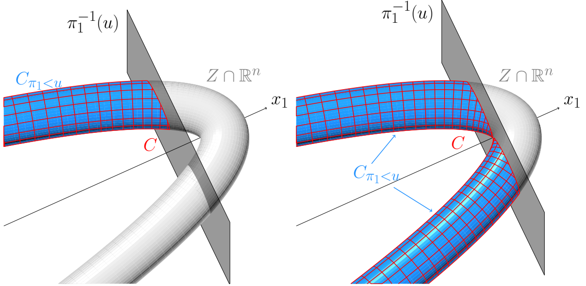
Figure 7: Illustration of Corollary 3.8 where \varphi = \pi_1 and Z is isomorphic to \mathbf{V}(x_1^2 + x_2^2 - 1) \times \mathbf{V}(x_1 + x_2^2) . On the left Z_{|\pi_1 = u} \cap K(\pi_1, Z) = \emptyset and one sees that C_{|\pi_1 < u} is still a semi-algebraically connected component of Z_{|\pi_1 < u} . On the right Z_{|\pi_1 = u} \cap K(\pi_1, Z) \neq \emptyset and one sees that C_{|\pi_1 < u} is disconnected.
