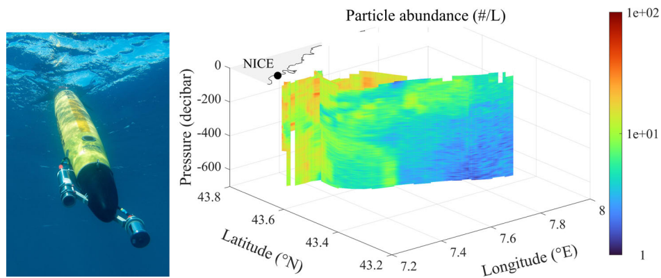
Fig. 7. Left: UVP6-LP mounted looking forward on a Seaxplorer glider, camera on the left and light on the right on the photo. Right: Abundance of particles from the 256 to 323 μm intermediate-size class provided as an example during a 71-dive deployment in the Mediterranean Sea off Nice, from 26 March 2019 to 29 March 2019. The glider transect was from the continental slope offshore.
