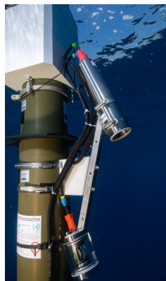
Fig. 6. Left: UVP6-LP mounted looking downwards on a NKE CTS5 BCG-Argo float. Right: The abundance of particles from the 256 to 323 \mu\text{m} intermediate-size class provided as an example during a 15-profile float deployment in the Mediterranean Sea off Nice. The float drifted along the steep continental slope from 20 November 2019 to 25 November 2019.
