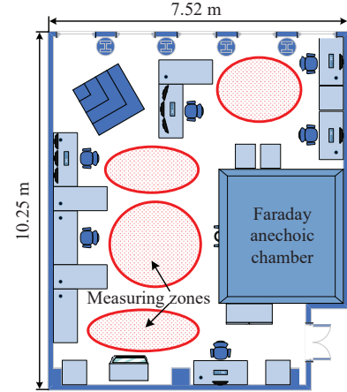
Fig. 9. Floor plan of the measuring scenario.
