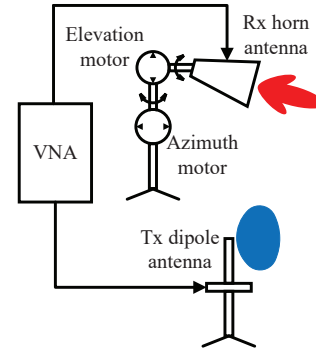
Fig. 10. Schematic of the experimental set-up.
