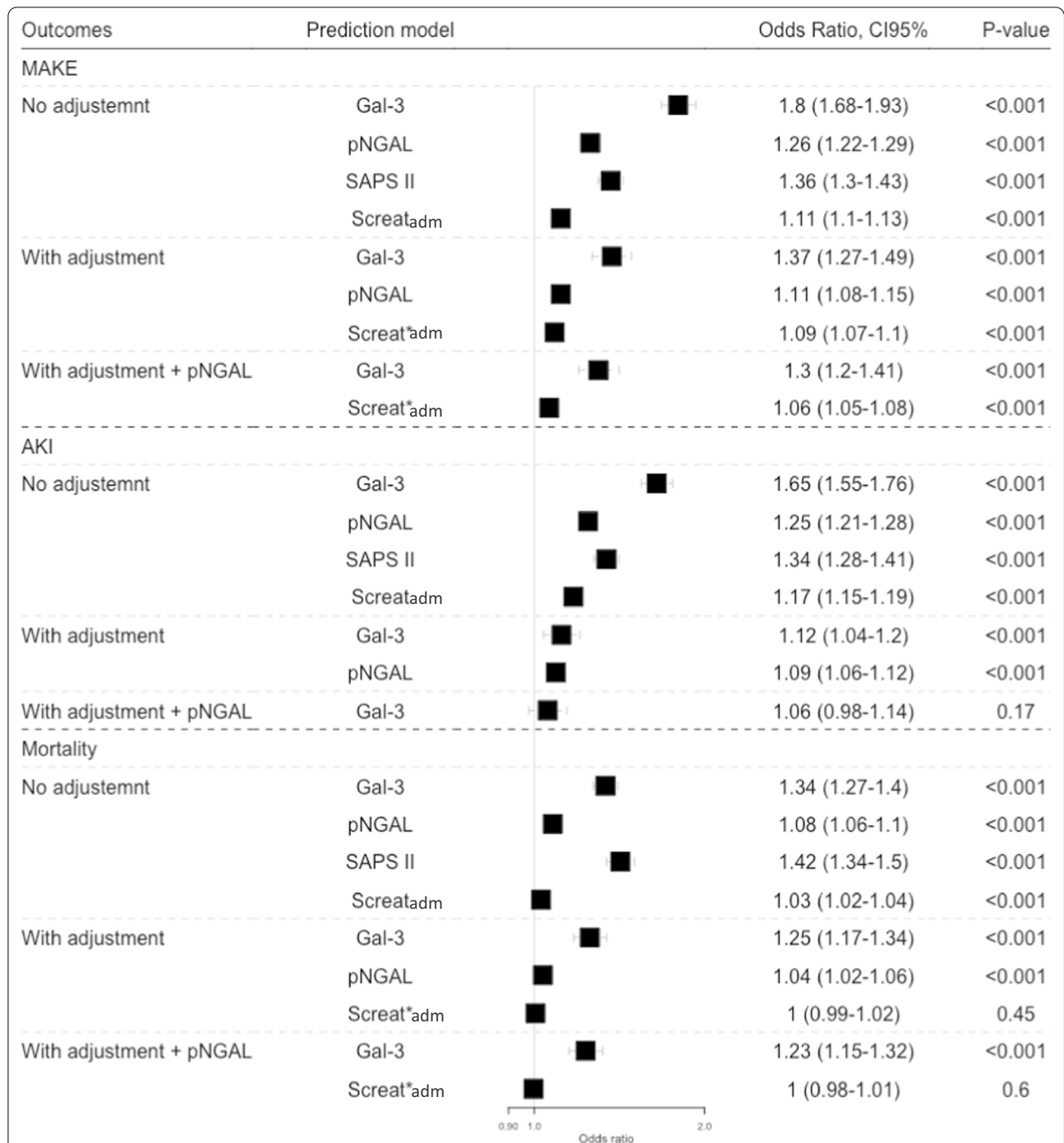
Fig. 2 Gal-3, SAPSII, Screat adm , pNGAL, Gal-3 after adjustment and Screat adm after adjustment, Gal-3 after adjustment including pNGAL and Screat adm after adjustment including pNGAL association with MAKE, AKI and Mortality. Gal-3 association was adjusted with gender, age, CKD, vasopressor treatment, SAPS II, Charlson score, Screat adm and lactate value at admission. For AKI association, Screat was not include in the adjustment model. OR for continuous variables (Gal-3, SAPSII, Screat adm ) were standardized for each 10-unit change, and pNGAL for each 100-fold unit change. *These model do not include Screat adm . OR, odds ratio; CI, confidence interval; SAPS II, Simplified acute physiology score II; MAKE, Major adverse kidney event; Gal-3, galectin 3; Screat, serum creatinine; CKD, Chronic kidney disease
