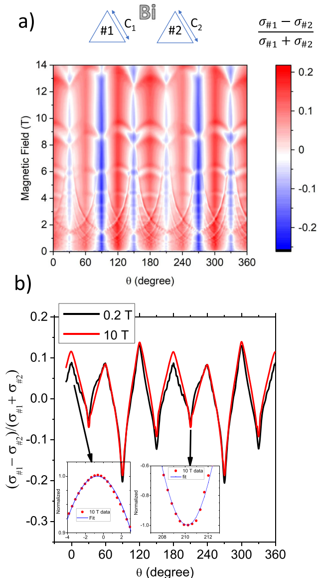
Fig. 5 Field and angle dependence of the excess boundary conductance. a Color plot of \frac{\sigma_{\#1} - \sigma_{\#2}}{\sigma_{\#1} + \sigma_{\#2}} at T = 1.55 K. Measurements were simultaneously performed for both samples in a fixed magnetic field at intervals of 0.1 T between 0 and 14 T. Values of \frac{\sigma_{\#1} - \sigma_{\#2}}{\sigma_{\#1} + \sigma_{\#2}} were calculated at each pair of angle and field values and put into a matrix of 721 \times 141 dimensions. A commercial software (Origin from OriginLab Corp.) was used to generate the color contour map. Red and blue stripes represent the excess and the deficit of conductivity. b Angle dependence of \frac{\sigma_{\#1} - \sigma_{\#2}}{\sigma_{\#1} + \sigma_{\#2}} at B = 0.2 T and at B = 10 T. The relative deficit and excess conductivity caused by field-boundary alignment does not change significantly in spite of three orders of magnitude change in the amplitude of bulk magnetoconductance. The angle dependence also remains roughly identical for B = 0.2 T and B = 10 T. Insets in panel b show \cos(q\theta) fits to the data over a narrow angular window (see text).
