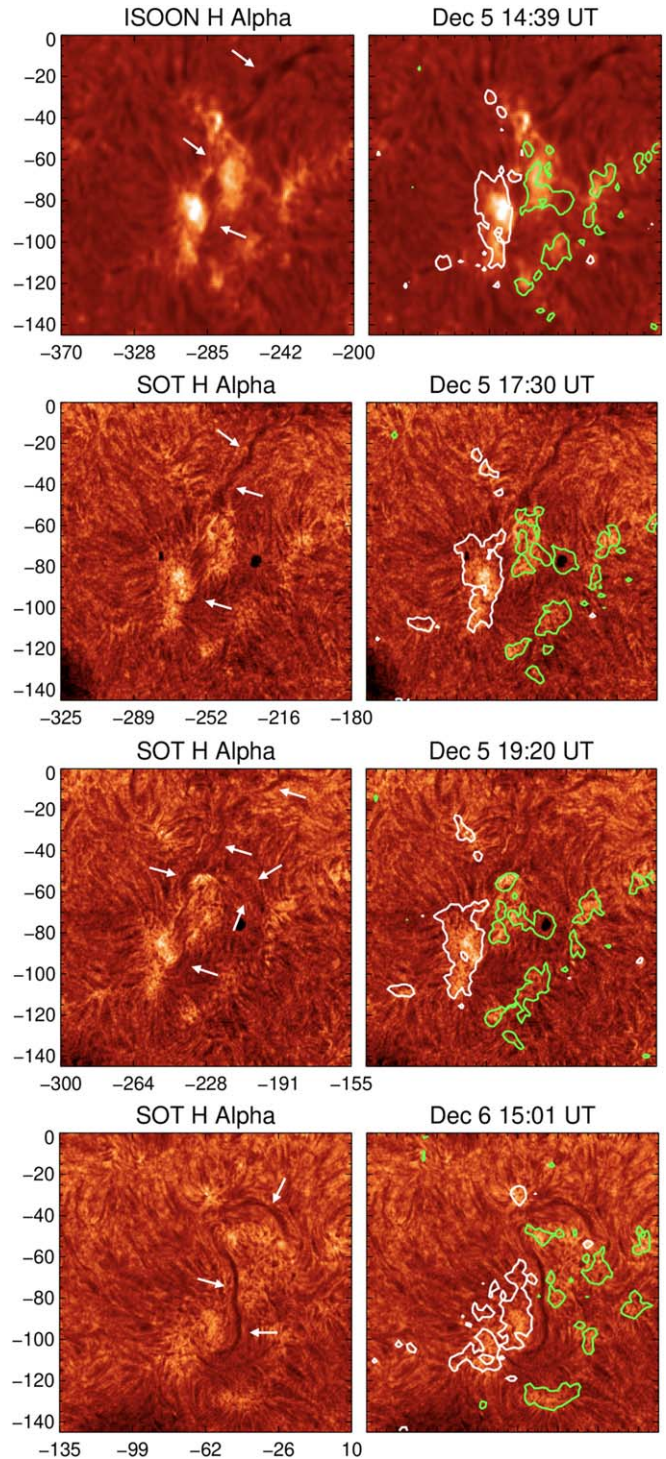
Figure 4. ISOON and Hinode/SOT H\alpha images at (a) 14:39 UT, (b) 17:30 UT, and (c) 19:20 UT on December 5 and at 15:01 UT on December 6 without/with contours (left/right) of SOHO/MDI line-of-sight magnetic field component of \pm 100 G (white/green for positive/negative values). Filaments are indicated by the white arrows. x and y coordinates are in arcsec.
