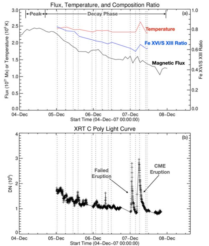
Figure 1. Global evolution of AR 10977. (a) Half of total unsigned flux (black), mean temperature (red), and mean Fe XVI 262.98 Å/S XIII 256.69 Å composition ratio (blue) vs. time. Hinode/EIS raster start times are shown with dashed gray lines. The global evolution of magnetic flux, temperature, and composition ratio are compared in Section 5.5. (b) Hinode/XRT C-Poly light curve for December 5–7.
