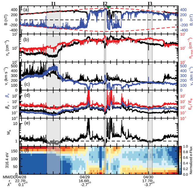
FIG. 1. An overview of the eighth solar encounter (E8) by PSP. (a) Total amplitude ( B , black) and radial component ( B_r , blue) of magnetic field, enveloped by the scaled B prediction (red). The green triangle indicates a perihelion at 15.9R_\odot on 29 April 2021 at 08:48 UT. (b) Electron density ( n_e , black) and the expected proton density ( n_{p\text{expt}} based on speed and distance, red). (c) Proton radial speed ( v_r , black) and the Alfvén speed ( v_A , blue). (d) Proton ( \beta_p , black) and electron ( \beta_e , blue) plasma beta together with the kinetic to magnetic energy density ratio ( E_k/E_B , red). (e) Radial Alfvén Mach number ( M_A ). (f) Normalized electron pitch angle distribution at 316.4 eV. The date (month/day), distance r , and latitude \lambda^\circ relative to the solar equator are indicated at daily intervals. PSP was in sub-Alfvénic flow for three periods in this encounter as shown by the shaded regions.
