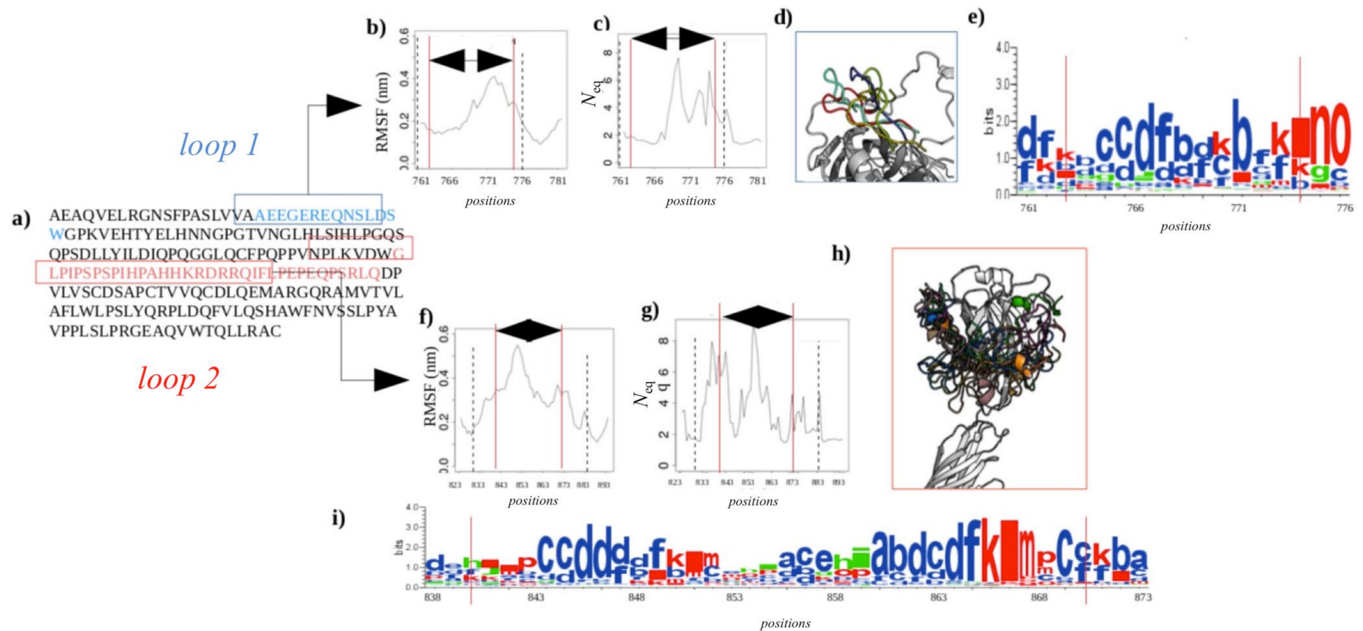
Figure 6. Calf-2 completed loops. (a) Sequence of the Calf-2 domain: in blue: the first completed loop; in red: the second one. (b,f) show the RMSF values for two loops. (c,g) show the N_{eq} values for the two loops. (d,h) are the 3-D representation of different conformations of the two modeled loops. (e,i) show the conservation logo maps of these two loops. The red lines on the graphs indicate the boundaries of the completed loops and in black dot lines the limits of entire loops.
