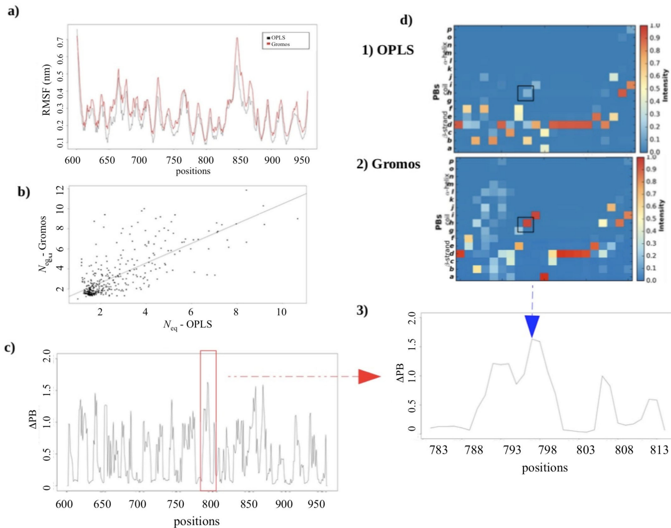
Figure 5. OPLS ff vs. Gromos ff. (a) RMSF and (b) Correlation between the N_{eq} values of each residue in Calf-1 simulated with OPLS ff ( x -axis) to Calf-1 simulated in Gromos ff ( y -axis). (c) \Delta PB between the simulations performed in these two forcefields. (d) PBs occurrence map [29] of positions 783 to 813 for (1) OPLS ff, and (2) Gromos ff, with corresponding (3) focused \Delta PB profile.
