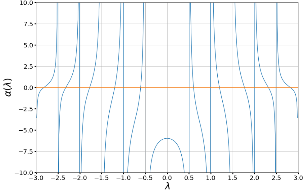
Figure 1: Secular function for \omega_c = 0.5 and n = 1
