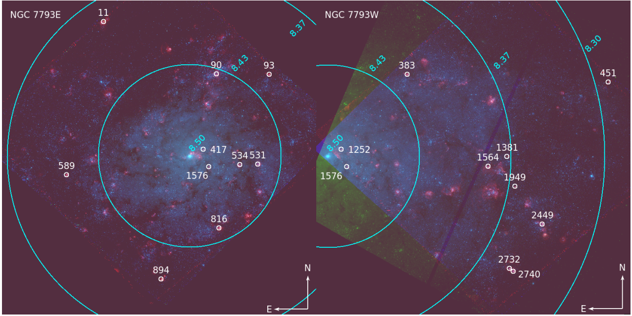
Figure 8. Composite RGB images of the partially-overlapping fields NGC 7793E (left panel) and NGC 7793W (right panel), where red = continuum-subtracted H\alpha , green = F555W, and blue = F438W. We use white circles to indicate the positions of the star clusters in our sample and give their LEGUS ID. In both images, the centre of the galaxy appears as a cyan knot. We overlay cyan circles centered on this knot, of radii equal to 0, 1, 2, and 3 arcmin. The value of 12+\log(O/H) in the ionized gas at each of these radii is shown with cyan characters. At 3.44 Mpc (Pietrzyński et al. 2010), 1 arcmin is \sim 1 kpc. Note that clusters 93 and 383, and 417 and 1252 have similar coordinates and photometry but have different IDs (see Section 4.3 for a discussion of these clusters). Also note that cluster 1576 appears in both fields and is at the edge of the H\alpha image for field NGC 7793W.
