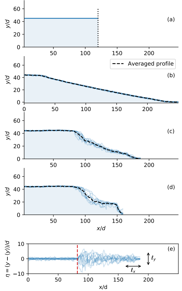
Fig. 1 Fluctuation of the final deposits around their mean profile. Blues lines : 10 simulations made in the same configuration, but varying the initial state. Dashed black line : average profile over the 10 simulations. (a) Initial column. (b) Final deposit. Bo = 0 . (c) Final deposit. Bo = 20 . (d) Final deposit. Bo = 50 . (e) Deposit profiles subtracted by their average over 10 collapses for Bo = 20 . Dashed red line: limit between static grains and flowing grains. The longitudinal length \ell_x and the transverse length \ell_y are sketched.
