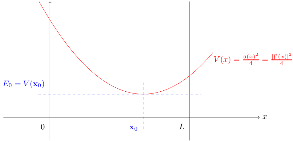
Figure 1: Geometric setting of Assumption 1.2
