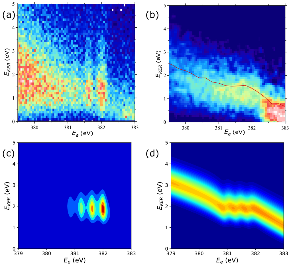
Fig. 9 2D plots for the distributions of E_{KER} as a function of resonant Auger electron energy E_e for the fragment band region. (a) Experimentally derived E_{KER} as a function of E_e measured at the top of the resonance, at \hbar\omega=400.66 eV. (b) Experimental data derived from the normalised momentum distribution as a function of E_e . The normalisation was done by the area for each bin of electron kinetic energy E_e . The red curve is the E_{KER} distribution, derived from the median momentum of the \text{NH}_2^+ ion (see Fig. 7). The observed intensity at E_e > 382.5 eV corresponds to the high-binding-energy tail of the molecular participator state e^- of \text{NH}_3^+ . (c) Theoretical cross section calculated by eq. (8) displaying four vibrational lines with the tails dispersing as E_e = \text{const} in agreement with the experimental panel (a). (d) Normalised theoretical cross section \sigma_{norm}^{fragm}(E_e, E_{KER}, \omega) (12) featuring that the dispersion of the tails of the vibrational line v=0 at E_e > 382 eV is close to E_{KER} + E_e = \text{const} in agreement with the experimental panel (b) and Fig. 7. Calculations were performed for v_c=0 , v_f=0, 1, 2, 3 , \Omega=0 , \Gamma = \text{HWHM} = 0.11 eV, P_{00}=0.4 , P_{01}=0.3 , P_{02}=0.2 , P_{03}=0.1 . \Gamma is the experimental HWHM broadening of the RAS vibrational lines. In simulations, we used experimentally derived dependence \gamma_{inst}(E_{KER}) = 0.09 + 0.282 \cdot E_{KER}^{0.6} .
