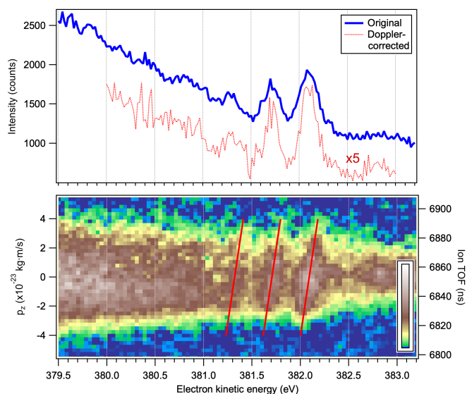
Fig. 6 Top panel: resonant Auger electron spectrum following the N\ 1s \rightarrow 4a_1 excitation at the top of the resonance, at \hbar\omega=400.66 eV. The blue curve corresponds to all detected electrons and the red curve to the electrons detected in coincidence with a single \text{NH}_2^+ ion and corrected for the Doppler energy shift. Bottom panel: Electron-ion coincidence (PEPICO) map of the Auger electrons and the \text{NH}_2^+ ions. The tilted red lines were derived using a purely analytical expression for the Doppler shift (eq. 4). The vertical scales give the flight times of the ions (right) and the corresponding values p_z of the ion momenta projected on the TOF spectrometer's axis (left).
