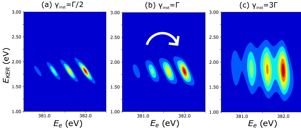
Fig. 10 Theoretical 2D plots of E_{KER} as a function of E_e calculated by eq. (8): the dispersion of vibrational lines 'rotates' clockwise with increase of the ratio \gamma_{inst}/\Gamma (see text for more details).
