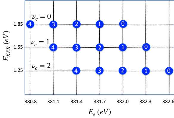
Fig. 8 Distribution of maxima of the total cross section \sigma^{fragm}(E_e, E_{KER}, \omega) (eq. 8) in the (E_{KER}, E_e) plane. Labels in circles show the vibrational quantum number of the final state v_f = 0, 1, 2, 3, 4 . Calculation is performed using eq.(11) for \nu_c = 0, 1, 2 and harmonic potentials for core-excited and final states with vibrational frequencies \omega_{vib} = 0.385 eV. \omega_{cf} = 382 eV. \Delta = 1 , \Delta E_c = E_c(R_0) - E_c(\infty) = 2 eV, \Omega = 0 . When \nu_c increases the distribution is shifted to the right (to higher values of E_e = \omega_{cf} + \varepsilon_{\nu_c} - \varepsilon_{v_f} , while E_{KER} = -\varepsilon_{\nu_c} + \Delta E_c + \Omega decreases (see eq. (11)).
