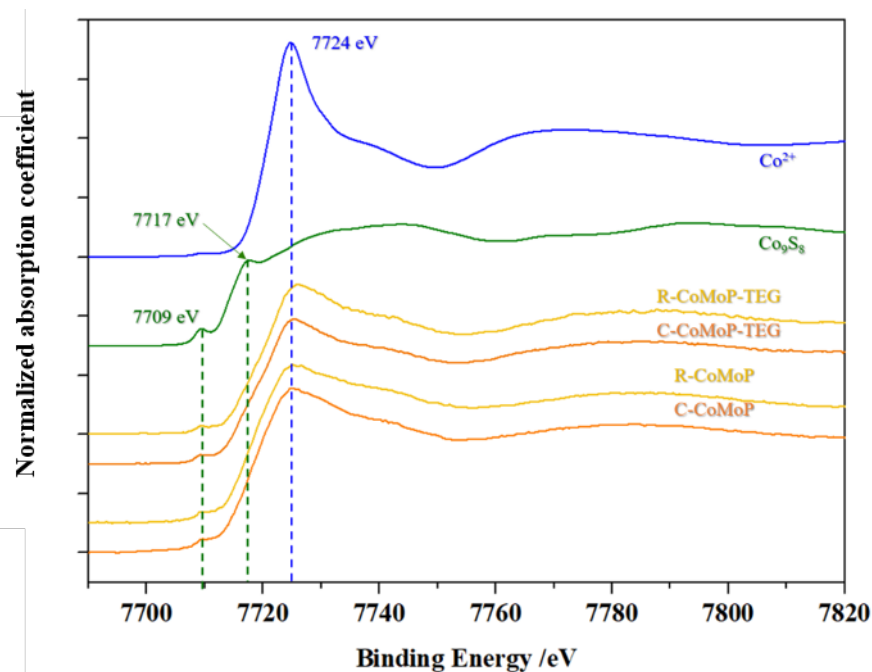
Figure 3. XANES Co K-edge spectra of model dried CoMoP and CoMoP-TEG catalysts supported on the C(0001) and R( 1\bar{1}02 ) planes of \alpha -Al 2 O 3 prepared by impregnation and sulfided at 300 °C. Spectra were acquired in a parallel orientation of the electric field vector of the synchrotron beam relative to the wafer surface.
