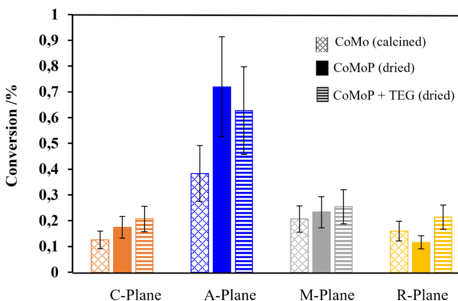
Figure 7. Thiophene conversion towards hydrodesulfurization products for model calcined CoMo [23] as well as dried CoMoP and CoMoP + TEG HDS catalysts supported on the C(0001), A(11 \bar{2} 0), M(10 \bar{1} 0) and R(1 \bar{1} 02) crystal planes of \alpha -Al 2 O 3 sulfided at 400 °C. Reaction conducted at 400 °C for 24 hours. Each catalyst exhibits the same exposed total area (four single crystals) and similar metal surface concentrations. Error bars of CoMoP and CoMoP-TEG samples correspond to the standard deviation over two to five measurements obtained for calcined CoMo catalysts. [23]
