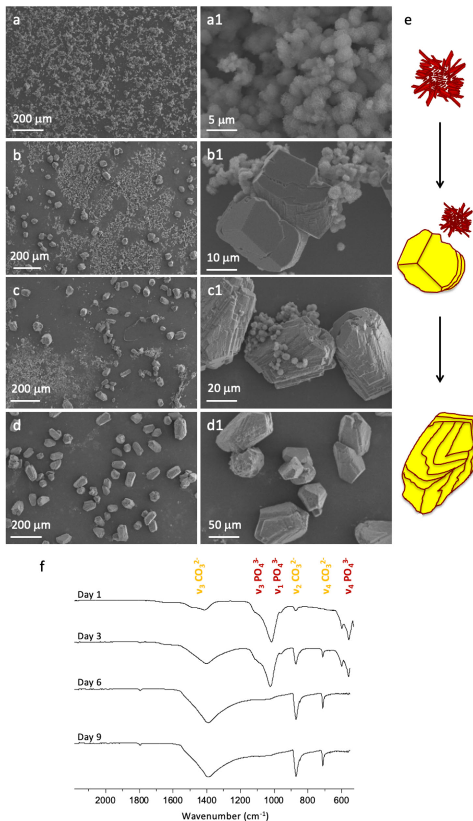
Fig. 5 Temporal evolution of minerals formed in the presence of inorganic phosphate with \text{Ca/P} = 3 . SEM images show the minerals formed after 1 day (a-a1), 3 days (b-b1), 6 days (c-c1), and 9 days (d-d1). The schematic representation of apatite evolution towards calcite with eroded surfaces is showed in (e). FTIR spectra of minerals formed after different reaction time (f).
