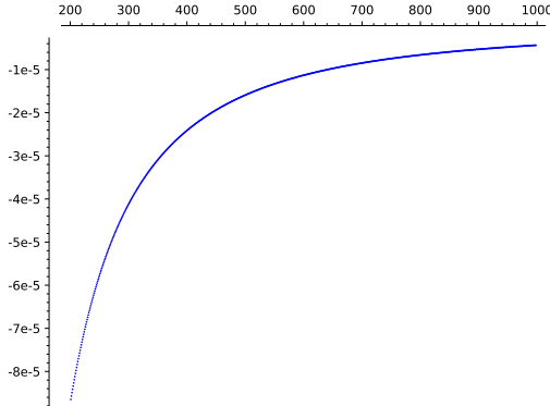
Figure 5.3. Plot of m(P_d) - m(P_\infty) , for 200 \leq d \leq 1000 . The SAGEMATH code we used to produce this plot is available online [32].
