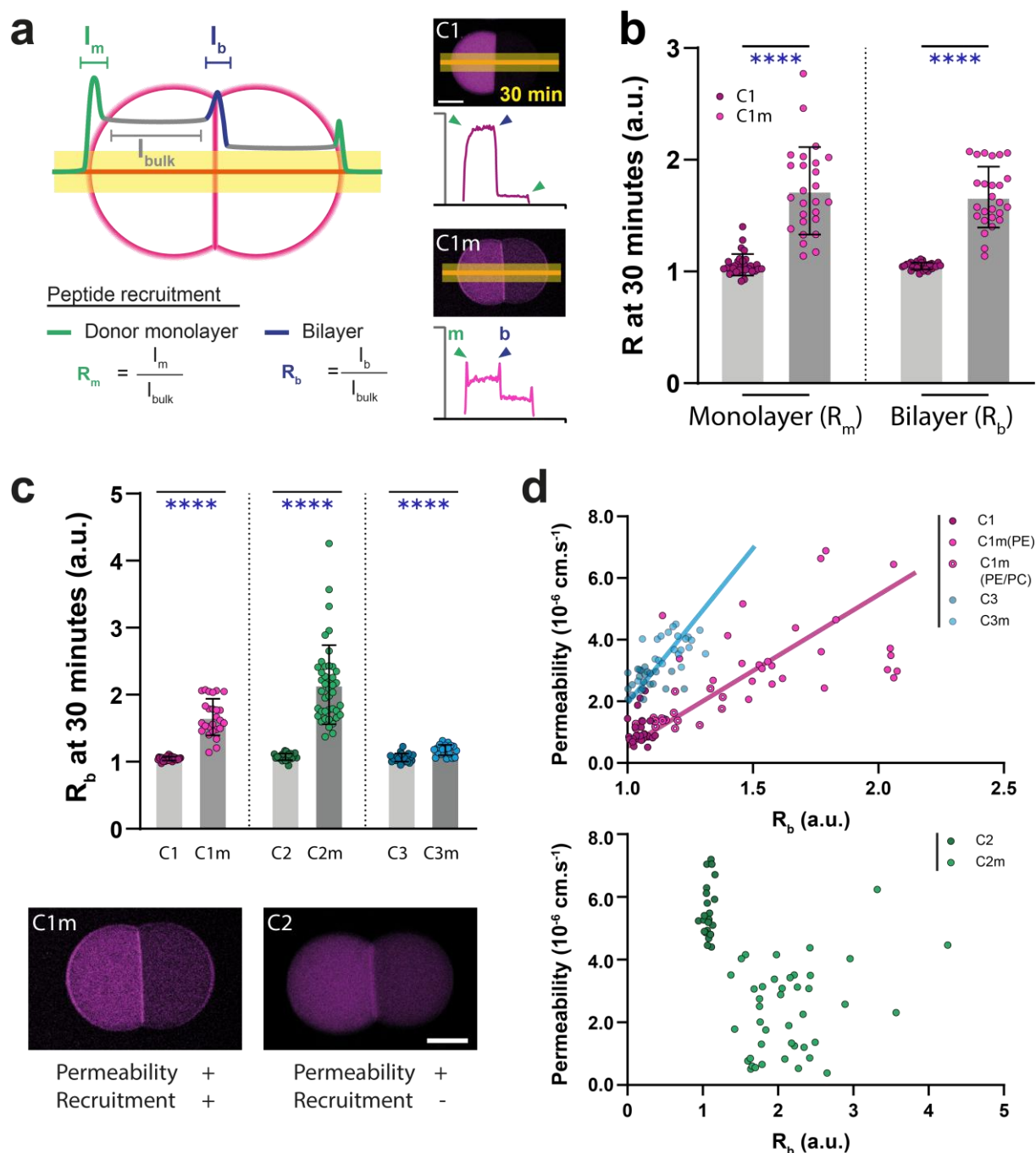
Figure 6: a) Schematic representation of DIB and the associated method to obtain fluorescence profile and peptide recruitment R_m and R_b . Scale bars, 100 \mu\text{m} . b) Monolayer donor ( mD ) and bilayer ( b ) recruitment values for peptides C1 and C1m. c) Bilayer recruitment values R_b for all three peptide couples (C1, C1m, C2, C2m, C3, C3m) d) Permeability value for each DIB assays as a function of
