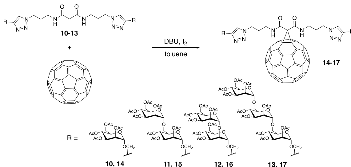
Scheme 3. Preparation of glycosylated fullerenes 14–17 .
