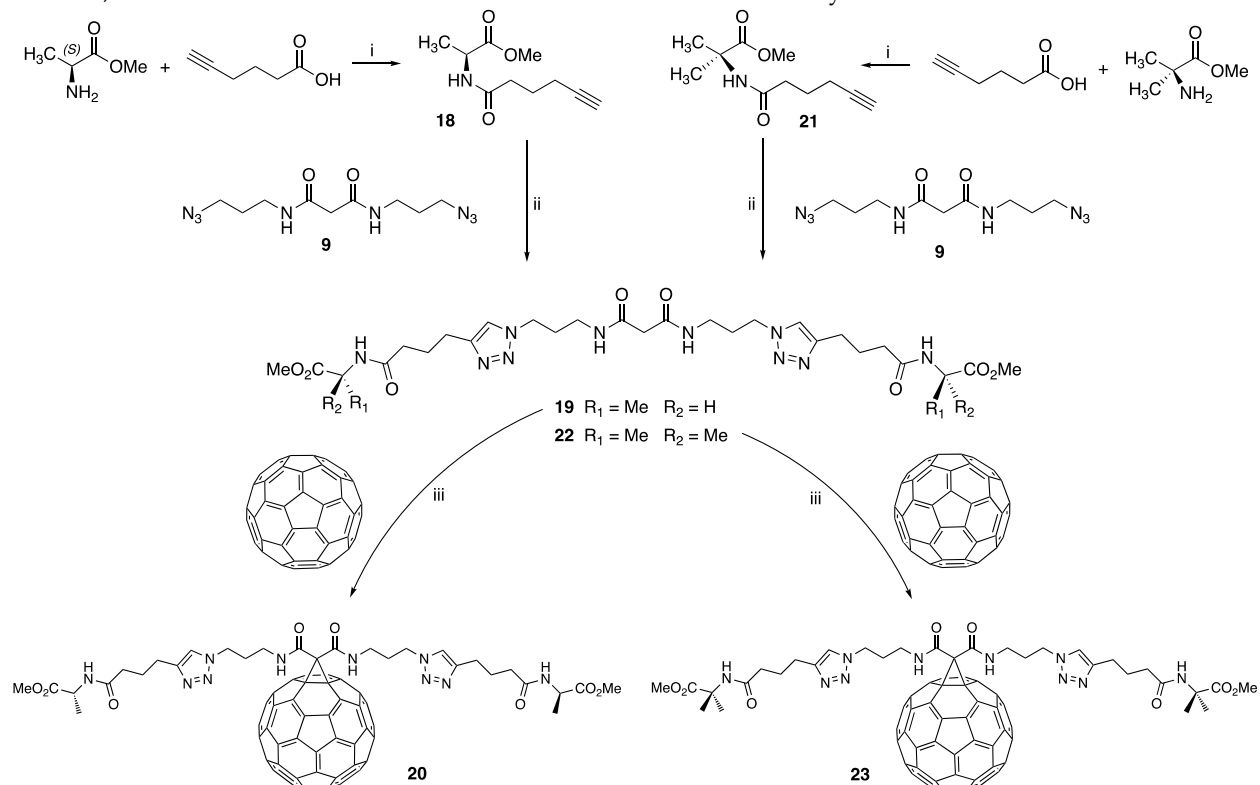
Scheme 4. Synthesis of amino acid-functionalized fullerenes. Experimental conditions: (i) DMAP, EDC HCl, DCM, 0 °C to rt, 16.5 h ( 18 = 90%; 21 = 75%); (ii) CuSO_4 , Na ascorbate, THF/ H_2O , overnight ( 19 = 70%; 22 = 98%); (iii) DBU, CBr_4 , toluene/ CHCl_3 (4:1) ( 20 = 20%; 23 = 25%).
