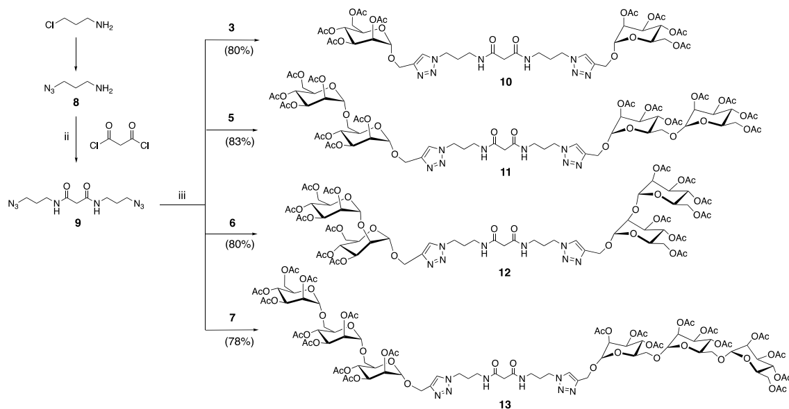
Scheme 2. Synthesis of sugar-modified malondiamide linkers. Experimental conditions: (i) 3-chloro propylamine, \text{NaN}_3 , \text{H}_2\text{O} , 80^\circ\text{C} , 6 h (91%); (ii) malonyl chloride, aqueous \text{NaOH} , \text{CH}_3\text{Cl} , 0^\circ\text{C} , 20 min (44%); (iii) \text{CuSO}_4 , Na ascorbate, \text{THF}/\text{H}_2\text{O} , overnight.
