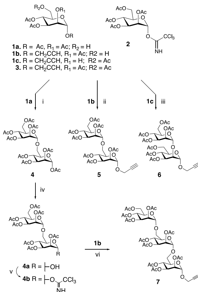
Scheme 1. Synthesis of propargyl-modified sugar derivatives. Experimental condition: (i) \text{BF}_3 \cdot \text{Et}_2\text{O} , dry DCM, 0 °C, 2.5 h (86%); (ii) \text{BF}_3 \cdot \text{Et}_2\text{O} , dry DCM, 0 °C to rt, 4 h (90%); (iii) \text{BF}_3 \cdot \text{Et}_2\text{O} , dry DCM, -50 °C to rt, 18 h (80%); (iv) hydrazine, DMF, 50 °C, 5 h (92%); (v) trichloroacetonitrile, DBU, dry DCM, 0 °C, 4 h (57%); (vi) \text{BF}_3 \cdot \text{Et}_2\text{O} , dry DCM, 0 °C, 4 h (56%).
