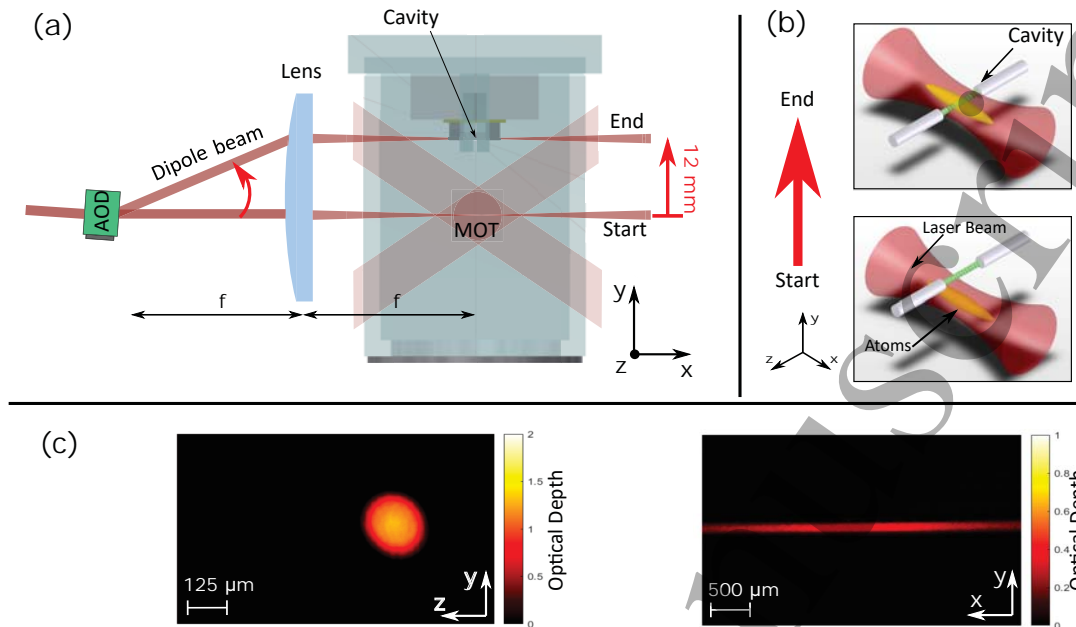
Figure 1. (a) The setup for transporting cold atoms from the MOT to the fiber microcavity. The method is based on a single-beam optical dipole trap at 1070 nm that moves due to an acousto-optical deflector (AOD). (b) Graphics showing the initial and final stage of the transport scheme. The optical trap (red) is moving the atoms (yellow) from below the cavity where the MOT is produced, up to the cavity where they can be transferred to the intra-cavity lattice (green). (c) Absorption images along two orthogonal directions of the atoms loaded in the dipole trap at the start of the transport after a time-of-flight of 0.5 ms (average over 10 single-shot images).
