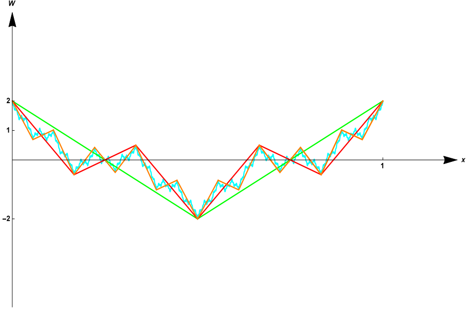
FIGURE 1.2. The graphs \Gamma_{W_0} , \Gamma_{W_1} (in red), \Gamma_{W_2} , \Gamma_W , in the case where \lambda = \frac{1}{2} , and N_b = 3 .
