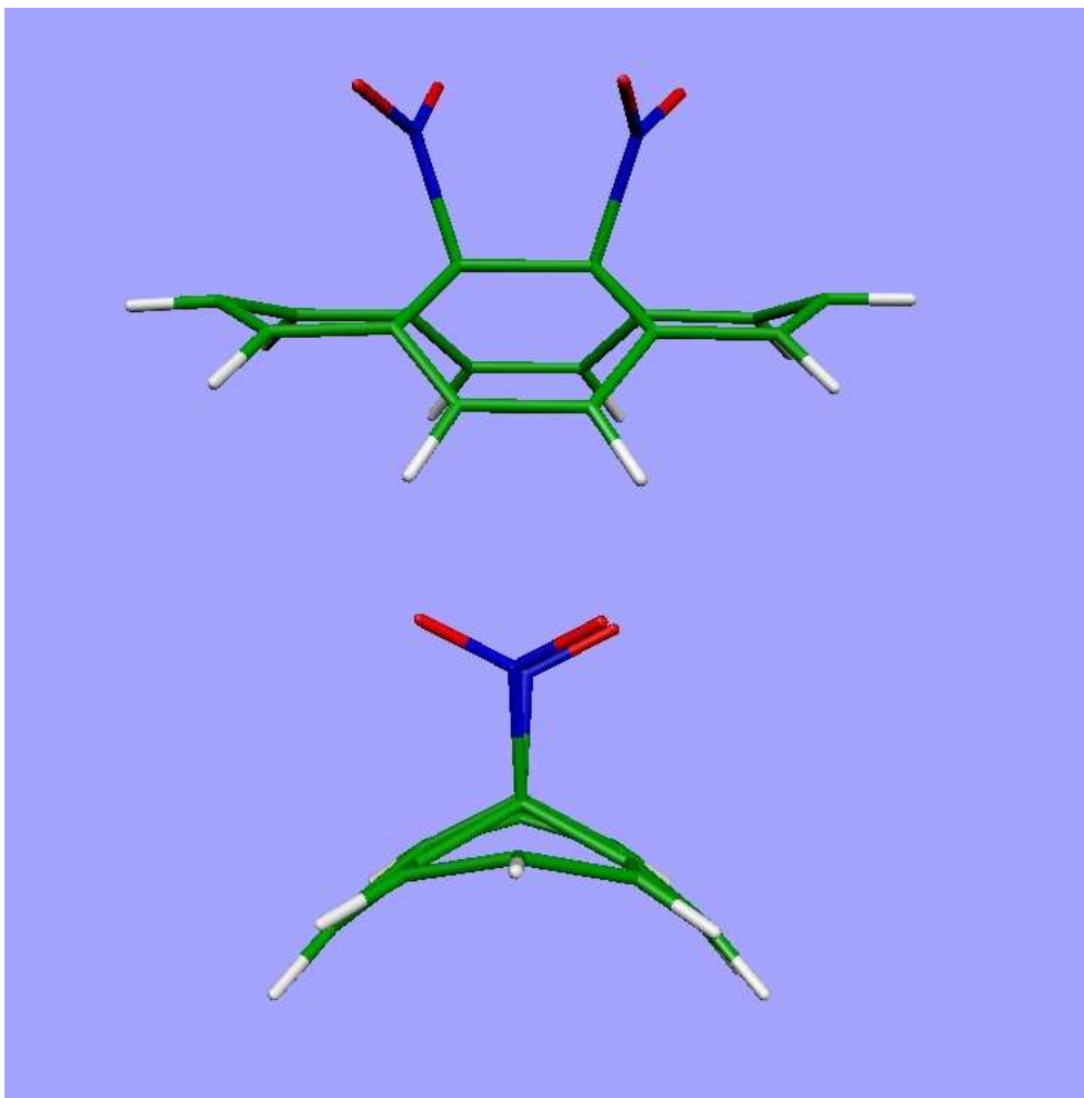
FIG. 1: Bonding configuration for \text{NO}_2 called “Ndown” where the N atoms are bonded to the nanotube model fragment.
