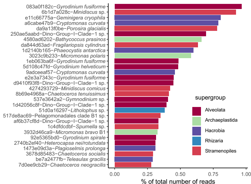
FIGURE 4 Protist V4 cASVs. (a) Most abundant cASVs (after normalization per sample). (b) Most frequent cASVs. Each cASV is coded by a 10-letter string representing the start of the 40-character hash value of the sequence (see Materials and Methods)
