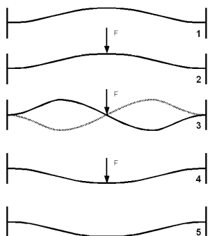
Figure 10. Snapping sequences for a typical clamped-clamped beam. Mode 2 buckling is used to help the switch from one position to the other.
