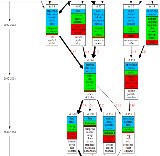
Figure 1: Pivot topics containing term “database” extracted from arXiv, green = emerging terms, blue = stable terms, red = decaying terms
