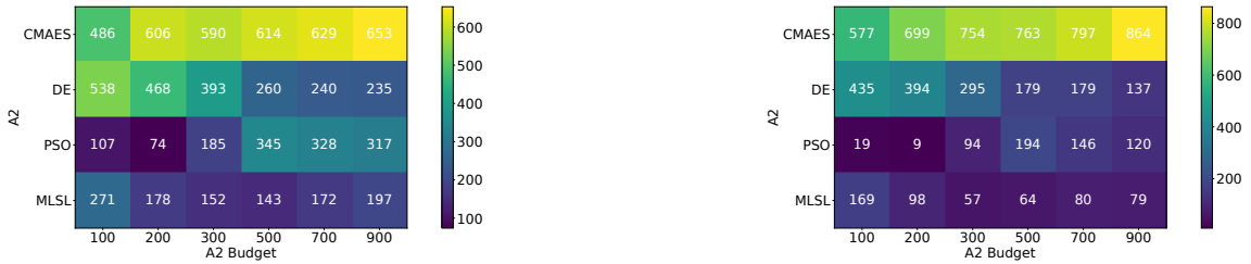
(a) How often each solver, excluding BFGS , is the best to switch to. (b) How often each solver, excluding BFGS , is actually selected.
