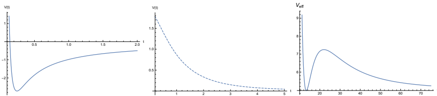
Fig. 1. Left figure: Vanishing of V(\tau) from 0^- happens for potentials with an AdS minimum. Middle: Large \tau behaviour of V(\tau) with power law correction \sim \frac{1}{\tau^n} . The potential on the right-hand side exhibits local minimum and maximum.
