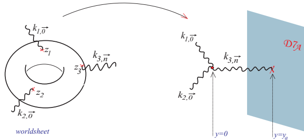
Fig. 2. Non-zero contribution from 1-loop; 3-graviton scattering amplitude of 2 massless gravitons and 1 KK mode corresponding to a closed string propagation in 2-dimensions towards a D7 brane.
