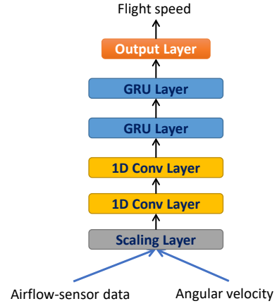
Figure 2: Neural network architecture
