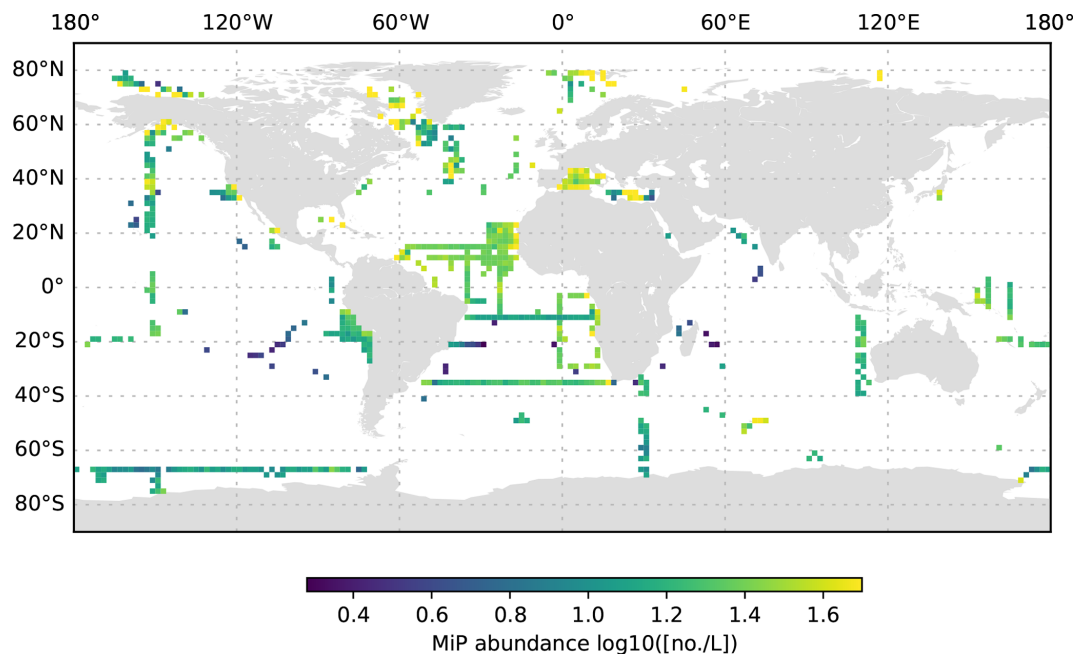
Figure 7. MiP abundance (decadic logarithm) averaged for the 200 to 1000 dbar depth layer and per 2^\circ grid box. Only profiles at least 1000 dbar deep were used for the analysis.
