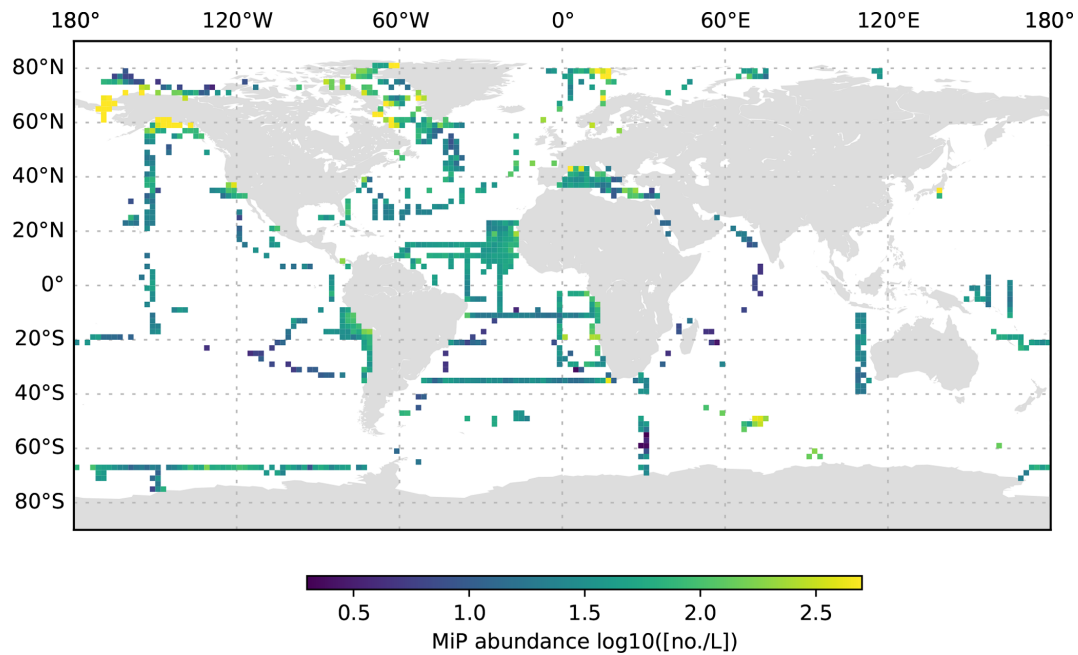
Figure 6. MiP abundance (decadic logarithm) averaged for the 0 to 200 dbar depth layer and per 2^\circ grid box. Only profiles at least 200 dbar deep were used for the analysis.
