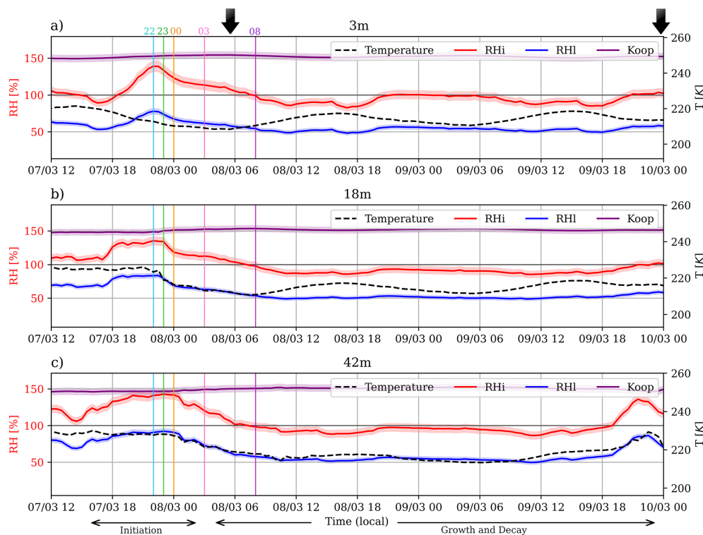
Figure 4. Time series of the temperature (dashed black line) and relative humidity with respect to ice (RHi, solid red line) and liquid water (RHI, solid blue line) at 3 (a), 18 (b) and 42 m a.g.l. (c). The red and blue shading shows the RH uncertainty ranges as estimated in Appendix A. The purple line shows the homogeneous freezing RHi threshold value of Koop et al. (2000). The 100 % RH value is highlighted with a solid black line. Vertical coloured bars indicate the times at which vertical profiles are analysed in Fig. 5. Black arrows indicate the times at which the fog visually appears and disappears near the surface in the lidar measurements.
