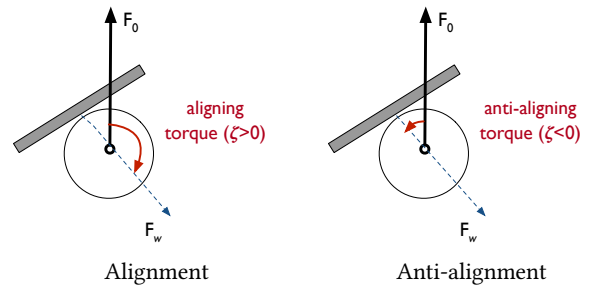
Figure 1: Illustration of the two variations of the active unit model, with F_0 the self-propulsive force and F_w the external force (applied from the contact point with the wall). Left: the unit's self-propulsive force aligns with the external force resulting from the collision (e.g. the unit escapes as soon as it no longer experience collision). Right: the unit's self-propulsive force anti-aligns with the external force, ultimately ending up with the unit facing the external force (e.g. the unit get stuck facing a the wall). See text for the full explanation.
