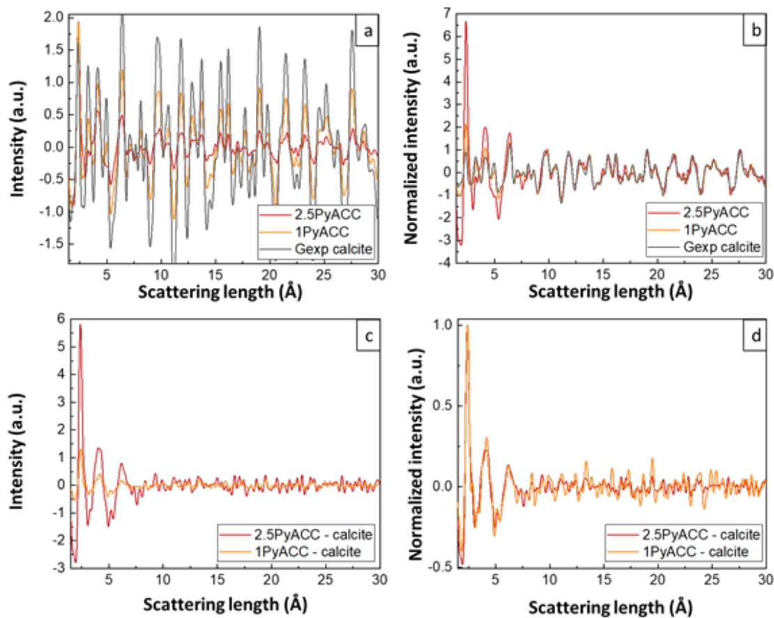
Figure S10: Comparison of the experimental G_{exp}(r) curves of 2.5PyACC, 1PyACC and calcite without normalisation (a) and after a normalisation by the 27.6 Å peak (b). G_{exp}(r)1PyACC - G_{exp}(r)calcite and G_{exp}(r)2.5PyACC - G_{exp}(r)calcite curves without additional normalisation (c) and with a normalisation by the first peak (d).
