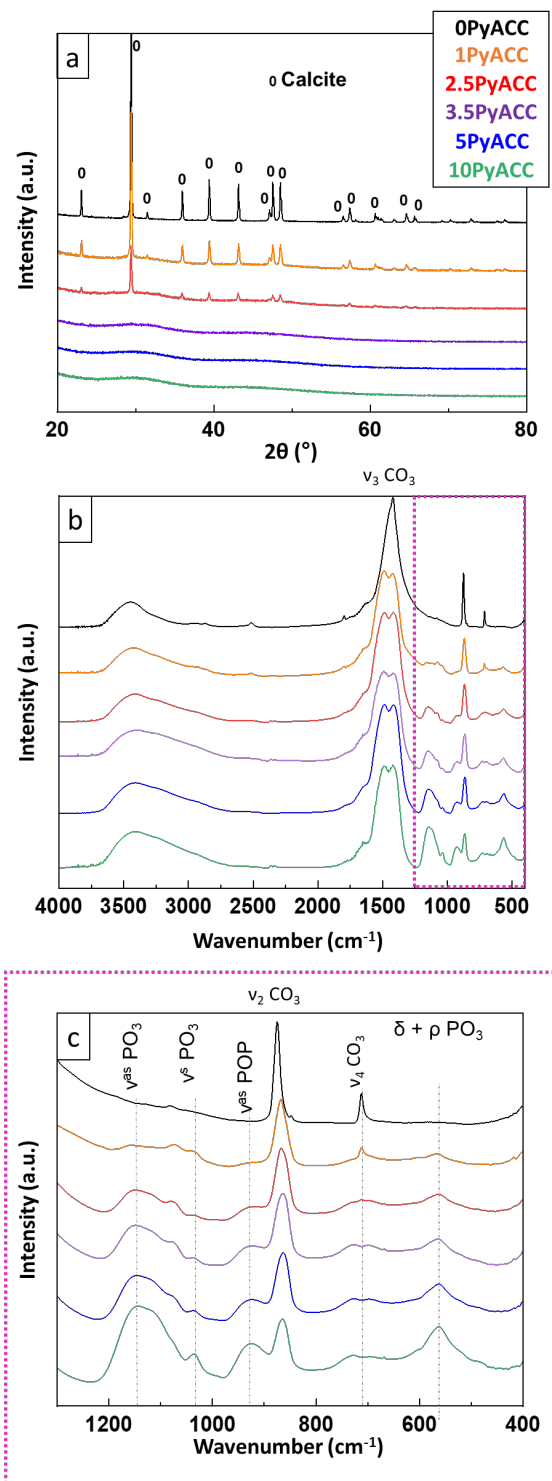
Figure 1: a) X-ray diffractograms of zPyACC powders synthesised in presence of various concentration of pyrophosphate. The narrow peaks are characteristic of calcite whereas the broad halo around 30^\circ was attributed to the amorphous structure. b) and c) Infrared spectra of zPyACC powders with identification of the vibrational bands of carbonate and pyrophosphate groups and in c) a zoom in the 400 - 1300 \text{ cm}^{-1} region (corresponding to the pink rectangle in Figure 1b).
