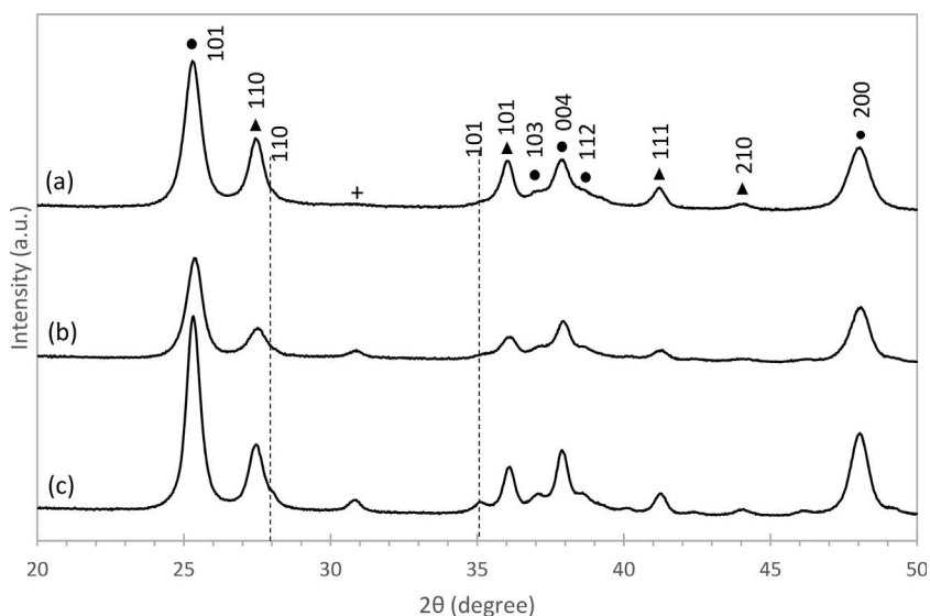
Fig. 5. XRD patterns of (a) (R + A)28, (b) (R + A)28-BA, (c) (R + A)28-AA from homemade supports; rutile \text{TiO}_2 ( \blacktriangle ), anatase \text{TiO}_2 ( \bullet ), brookite \text{TiO}_2 (+), and rutile \text{RuO}_2 (drawn as dotted lines) peak positions.
