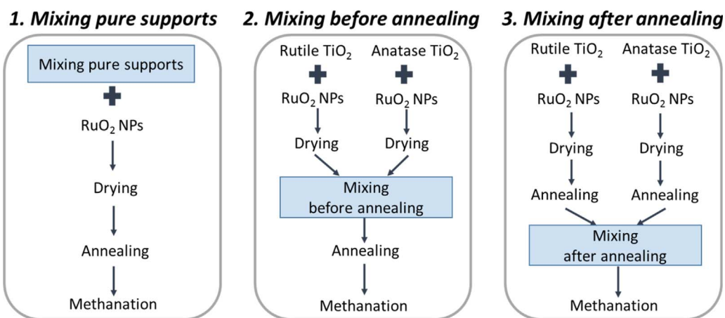
Fig. 1. Schematics of mixing anatase and rutile \text{TiO}_2 phases at different stages of catalyst preparation. The three routes are denoted “mixing 1”, “mixing 2” and “mixing 3” in the following. Methanation step include in-situ reduction of \text{RuO}_2 into Ru.
