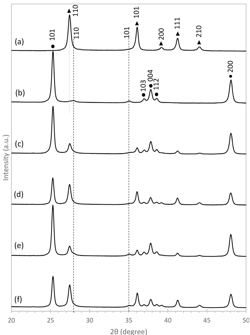
Fig. 10. XRD patterns of (a) CR100, (b) CA100, (c) C(R + A)28, (d) C(R + A)55, (e) C(R + A)28-AA, and (f) C(R + A)55-AA obtained from commercial supports; rutile \text{TiO}_2 ( \blacktriangle ), anatase \text{TiO}_2 ( \bullet ), and rutile \text{RuO}_2 (drawn as dotted lines) peak positions.
