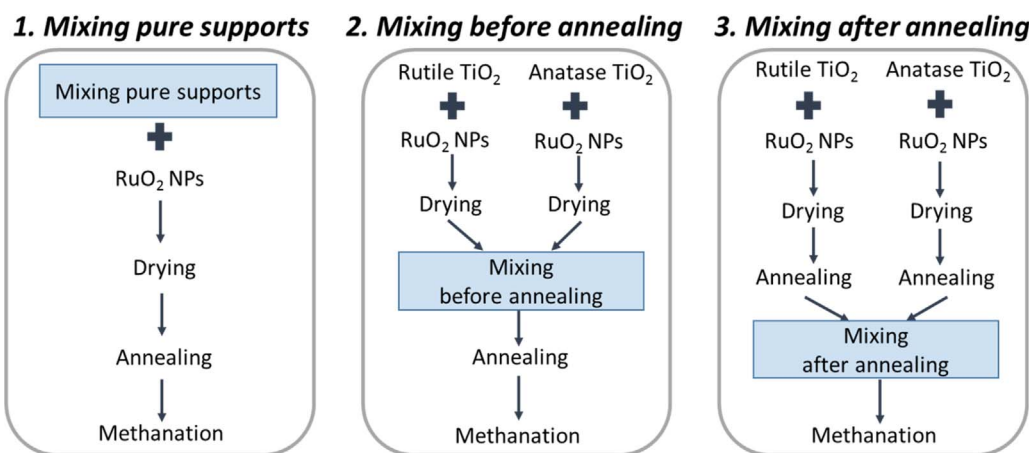
Fig. 1. Schematics of mixing anatase and rutile TiO 2 phases at different stages of catalyst preparation. The three routes are denoted “mixing 1”, “mixing 2” and “mixing 3” in the following. Methanation step include in-situ reduction of RuO 2 into Ru.
