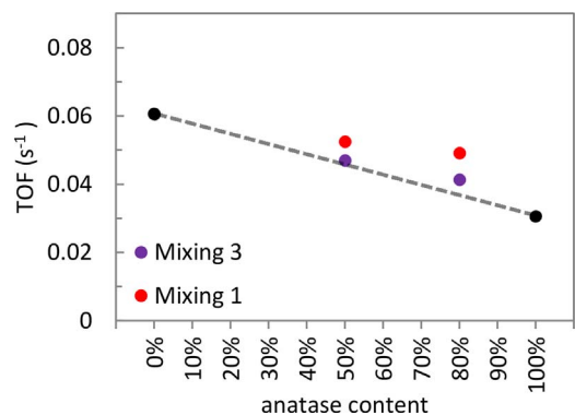
Fig. 12. Turn over frequencies (TOF) or methane production rates normalized per surface Ru probed by H 2 chemisorption for all catalysts concerned in this section. (For interpretation of the references to color in this figure legend, the reader is referred to the web version of this article.)
