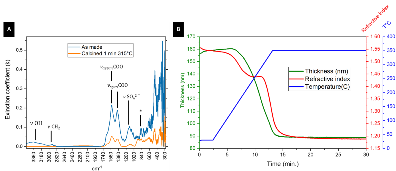
Figure 5 : (A) IR-VASE experiments on as-made and calcined three-layer thin film of \text{Gd}_2\text{O}_3\text{S} nanoparticles on Si/Ti/Cr substrates. (B) in-situ UV-NIR VASE experiment at 600\text{ nm} on a three-layer \text{Gd}_{1.9}\text{Ce}_{0.1}\text{O}_2\text{S} thin film on Si.
