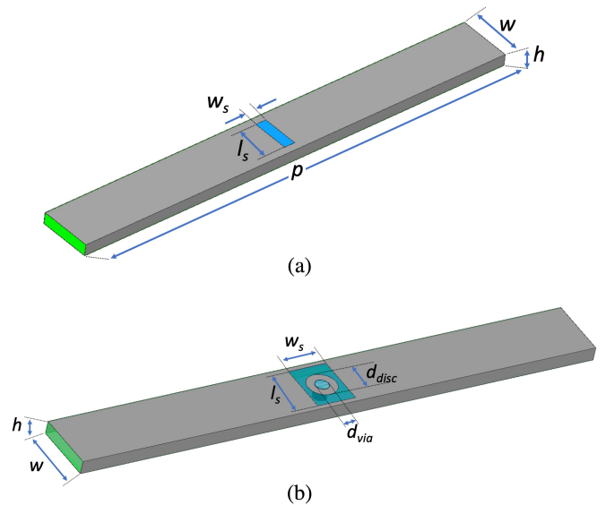
Fig. 1: Unit-cell ( w = 3.5 mm and h = 0.762 mm): (a) rectangular slot; (b) rectangular slot with via hole.
