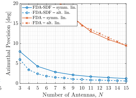
Fig. 4. Azimuthal precision of geocast delivery zone, for varying number of antennas N .
