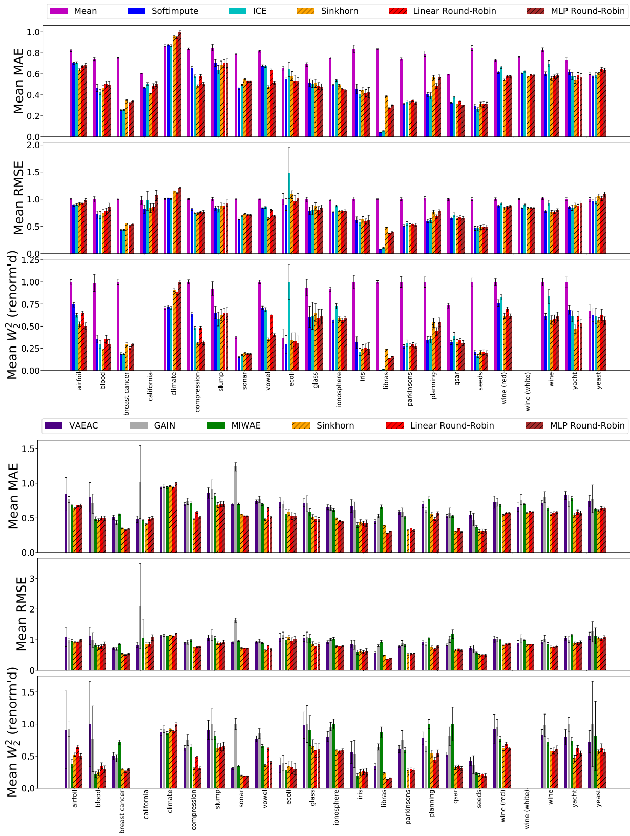
Figure 8: (30 % MCAR)
