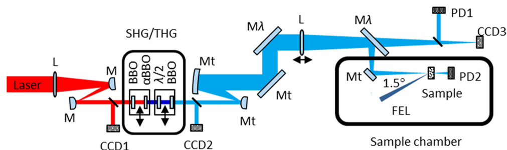
FIG. 4. Optical scheme of the TRIXS laser setup. The laser light propagates from left to right. L denotes focusing lenses; M are 800 nm mirrors; Mt are triple-band coated mirrors for 266 nm, 400 nm, and 800 nm; M\lambda are mirrors which are coated for a single wavelength, and need to be exchanged for different wavelengths; CCD1/2 are beam position monitor cameras; CCD3 is the virtual focus detector camera; and PD1/2 are photodiodes for monitoring the incoming laser intensity and for the time zero tool, correspondingly.
