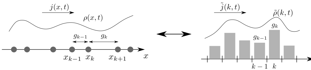
FIG. 2. Duality relation between two equivalent descriptions of a particle system: through the positions of the particles (left) and the through the gaps between the particles (right). The particle system is described at the macroscopic level by a density field \rho(x, t) and a current j(x, t) , while the dual system (gaps) is described by a density \tilde{\rho}(k, t) and a current \tilde{j}(k, t) . These two descriptions are equivalent, and related by Eqs. (27,28). The inverse transformation is identical, and written explicitly in Eqs. (30,31). These two sets of fields (\rho, j) and (\tilde{\rho}, \tilde{j}) obey the equations of fluctuating hydrodynamics (3,4), with transport coefficients respectively given by (D, \sigma) and (\tilde{D}, \tilde{\sigma}) , which are related by the transformation (29).
