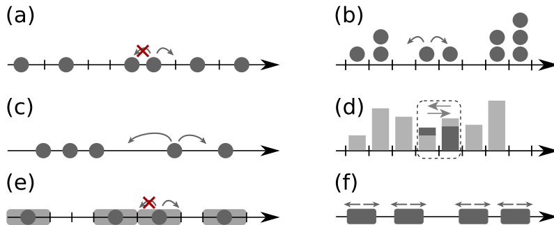
FIG. 4. The different models of single-file systems considered in this paper. (a) the simple exclusion process (SEP). Each particle can hop to a neighbouring empty site. (b) the zero range process (ZRP). The particles can hop on a neighbouring site. (c) the random average process (RAP). Particles on a continuous line can hop to a random fraction of the distance to the next particle. (d) the Kipnis Marchioro Presutti model (KMP). Each site hosts a continuous variable (a mass). At random times, the total mass of two neighbouring sites is randomly redistributed between them. (e) the double exclusion process. A particle can hop on a neighbouring site if the destination site and the next one is empty. It represents an exclusion process with particles that occupy the volume of two sites (shaded region). (f) the gas of hard rods. Particles of length \ell (rods) perform a Brownian motion, with the condition that the rods cannot overlap. The corresponding transport coefficients for these models are given in Table I.
