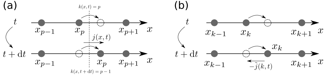
FIG. 3. (a) the flux j(x, t) of particles at position x at time t gives the variation of the index k(x, t) of the closest particle to the left of x , see Eq. (11). (b) The flux \tilde{j}(k, t) of gaps through particle k at time t gives the evolution of the position of this particle (13).
