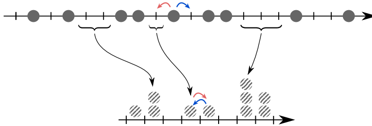
FIG. 1. Mapping of the simple exclusion process (SEP, top) onto the zero range process (ZRP, bottom) [20–22]. The particles of the SEP can hop on neighbouring sites, only if they are empty. The sites of the ZRP correspond to the particles of the SEP. The number of particles on a site in the ZRP is the number of empty sites on the right of the corresponding particle in the SEP. For the SEP, we have represented by two arrows the possible jumps of an individual particle. We have represented in the ZRP the corresponding dynamics, illustrated by the two arrows corresponding to the jumps of the SEP particle.
