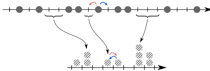
FIG. 1. Mapping of the simple exclusion process (SEP, top) onto the zero range process (ZRP, bottom) [20–22]. The particles of the SEP can hop on neighbouring sites, only if they are empty. The sites of the ZRP correspond to the particles of the SEP. The number of particles on a site in the ZRP is the number of empty sites on the right of the corresponding particle in the SEP. For the SEP, we have represented by two arrows the possible jumps of an individual particle. We have represented in the ZRP the corresponding dynamics, illustrated by the two arrows corresponding to the jumps of the SEP particle.
