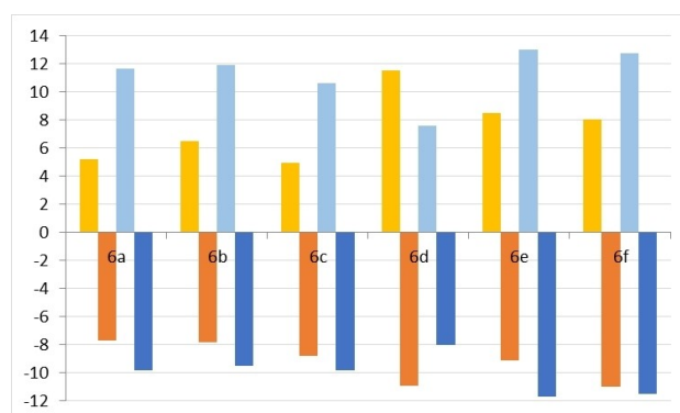
Figure 2. D/I AS analysis for the cycloaddition A-pathway (orange, left) and heterocycloaddition B-pathway (blue, right): \Delta E_{\text{dis}} global distortion (light colors, positive values) in kcal.mol -1 ; \Delta E_{\text{int}} interaction (dark colors, negative values), in kcal.mol -1 .
