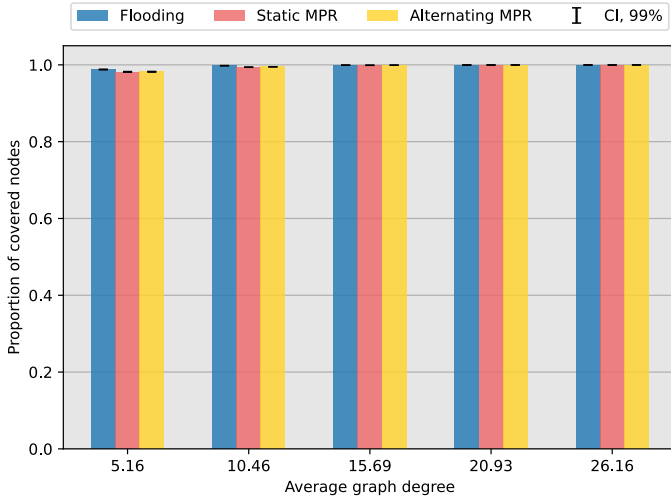
Fig. 6. Reachability
