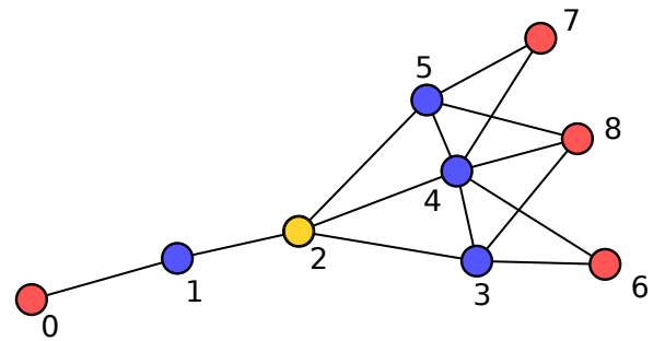
Fig. 2. Algorithm walkthrough
