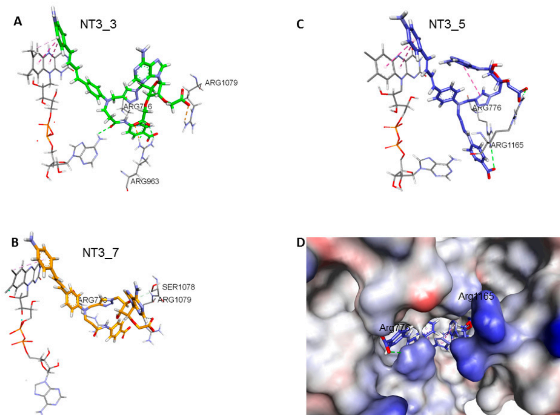
Figure 3. Comparison of NT3_5, NT3_7, NT3_3: effect of charge on key interactions between the nanotriggerers bound to eNOS. Representative structures of the 3 replicas (A) NT3_3, (B) NT3_7, (C) NT3_5 for clarity, the view emphasizes only interactions of the carboxylate groups with arginine residues of eNOS; the interactions between the NTs and eNOS are listed in Table 2 and their interaction energies summarized in Table 3; (D) solvent surface view of NT3_5 in the NADPH site; the view emphasizes R776 and R963 at the aperture of the site; FAD has been removed for clarity. Color code: blue positively interpolated charge, red negatively interpolated charge.
