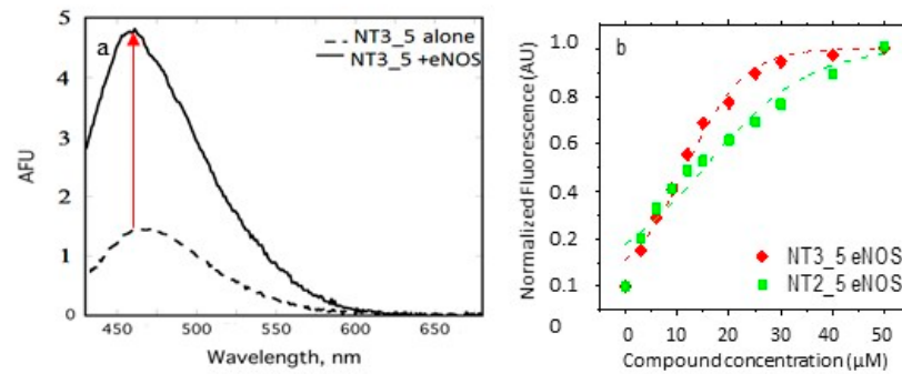
Figure A1. (a) Spectral changes of NT3_5 upon binding to eNOS. Fluorescence emission spectra were recorded from 430–680 nm (excitation = 420 nm; slit width = 5 nm) for NT3_5 (10 \mu M) alone and for eNOS (5 \mu M) + NT3_5 (10 \mu M). Spectrum of intrinsic protein fluorescence (due to flavins) was subtracted from protein+ NT spectrum. Fluorescence maxima were found at 470 nm and 450 nm for NT3_5 alone and eNOS + NT3_5, respectively, demonstrating an increase in fluorescence intensity and a blue shift upon binding to eNOS. (b) Titration of eNOS with NT2-5, NT3_5. Fluorescence emission spectra were recorded from 430–680 nm (excitation = 420 nm; slit width = 5 nm). Spectra of intrinsic protein fluorescence and unbound NT were subtracted from protein/NT spectra, and fluorescence at 460 nm was plotted. Representative data (out of four experiments in each NT) have been fitted by a single dose–response (NT2_5, NT3_5) (Table 1).
