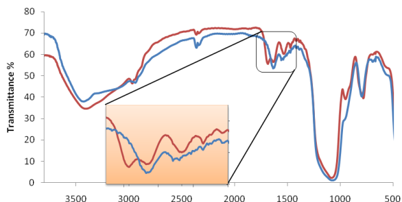
Figure 3. IR spectra of \text{NH}_2 -functionalized SBA-15 with 2.0\text{ mmol g}^{-1} (in red) and of POM anchored onto SBA-15 support (in blue).
