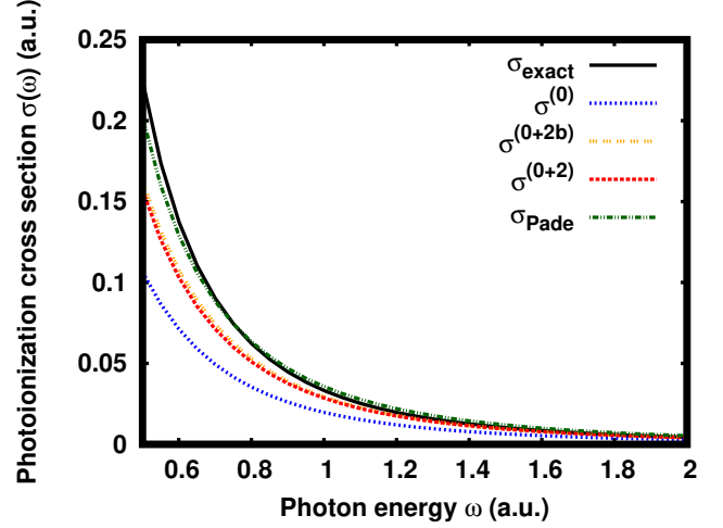
Fig. 1. Photoionization cross section of the hydrogen atom ( Z = 1 ). The exact cross section \sigma_{\text{exact}}(\omega) [Eq. (46)] is compared with the zeroth-order semiclassical approximation \sigma^{(0)}(\omega) [Eq. (42)], the partial second-order semiclassical approximation \sigma^{(0+2b)}(\omega) = \sigma^{(0)}(\omega) + \sigma^{(2b)}(\omega) [Eqs. (42) and (44)], the full second-order semiclassical approximation \sigma^{(0+2)}(\omega) = \sigma^{(0)}(\omega) + \sigma^{(2b)}(\omega) + \sigma^{(2c)}(\omega) [Eqs. (42), (44), and (45)], and the Padé approximant \sigma_{\text{Padé}}(\omega) [Eq. (48)].
