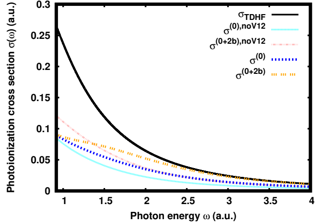
Fig. 3. Photoionization cross section of the helium atom ( Z = 2 ). The reference TDHF cross section \sigma_{\text{TDHF}}(\omega) [40, 9] is compared with the zeroth-order semiclassical cross section \sigma^{(0)}(\omega) [Eq. (60)] and the partial second-order semiclassical cross sections \sigma^{(0+2b)}(\omega) = \sigma^{(0)}(\omega) + \sigma^{(2b)}(\omega) [Eqs. (60) and (64)]. Also reported are the approximate zeroth-order and partial second-order semiclassical cross sections \sigma^{(0), \text{noV12}}(\omega) and \sigma^{(0+2b), \text{noV12}}(\omega) = \sigma^{(0), \text{noV12}}(\omega) + \sigma^{(2b), \text{noV12}}(\omega) [Eqs. (60) and (64)] in which the two-electron Coulomb interaction V_{12}(\mathbf{q}_1, \mathbf{q}_2) = 1/\|\mathbf{q}_1 - \mathbf{q}_2\| has been neglected.
